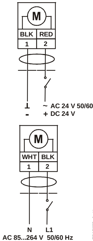
Figure 9: Control Wiring Diagrams
