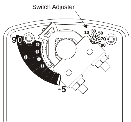
Figure 12: Switch Trip Point Settings
